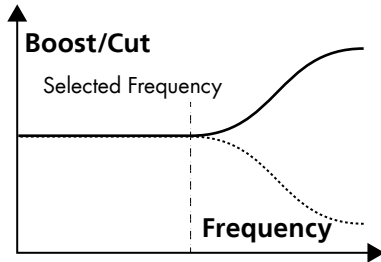
Figure 10.5 A high shelf EQ.
