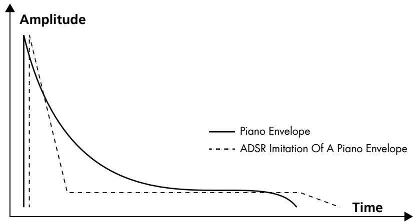
Figure 2.4 The ADSR type envelope may not be the ideal choice for piano type patches.
