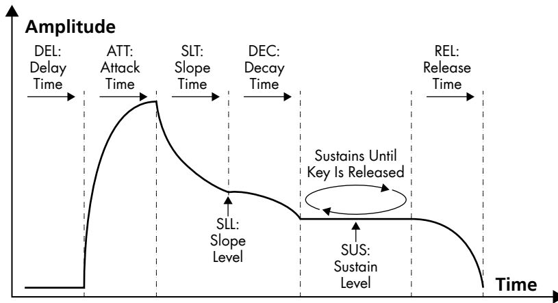
Figure 2.9 The envelope curves in Z3TA+.
