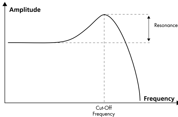
Figure 3.5 A low-pass filter with a resonant peak.
