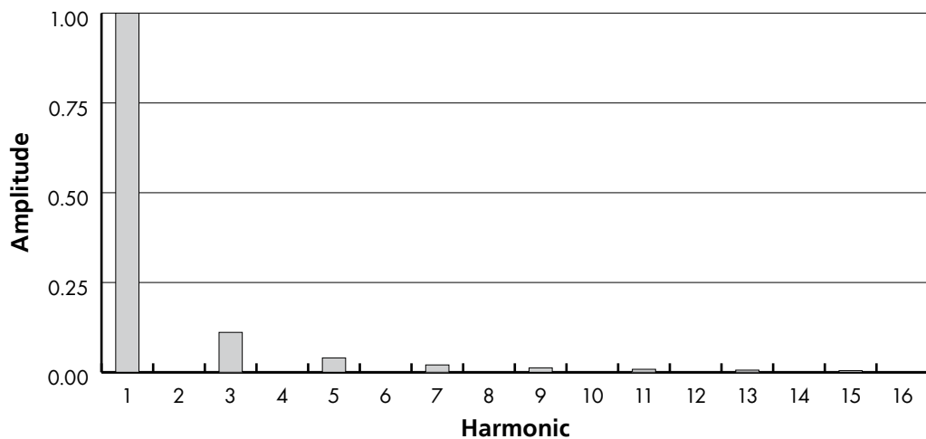
Figure 9.3 The first eight partials of a triangle wave.
