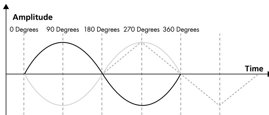
Figure 4.7 The phase of an oscillator. The gray sine wave has reversed polarity (when compared to the black sine wave) and the dotted triangle wave is 180 degrees out of phase.
