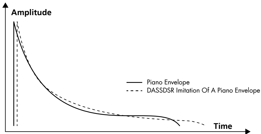
Figure 2.8 The Z3TA+ envelope gets closer to the envelope of a piano.
