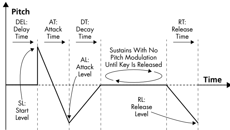
Figure 2.10 The Z3TA+ pitch envelope.
