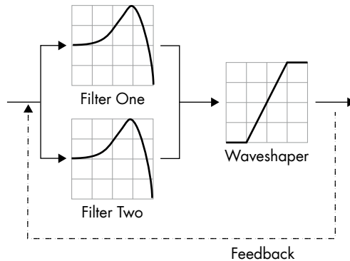
Figure 3.10 Dual option one arrangement of the filter section in Surge. This allows for two separate sounds to be created and processed through different filters.
