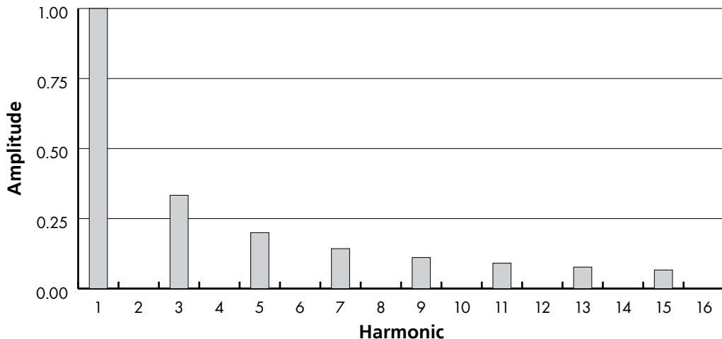
Figure 9.1 The first eight partials of a square wave.
