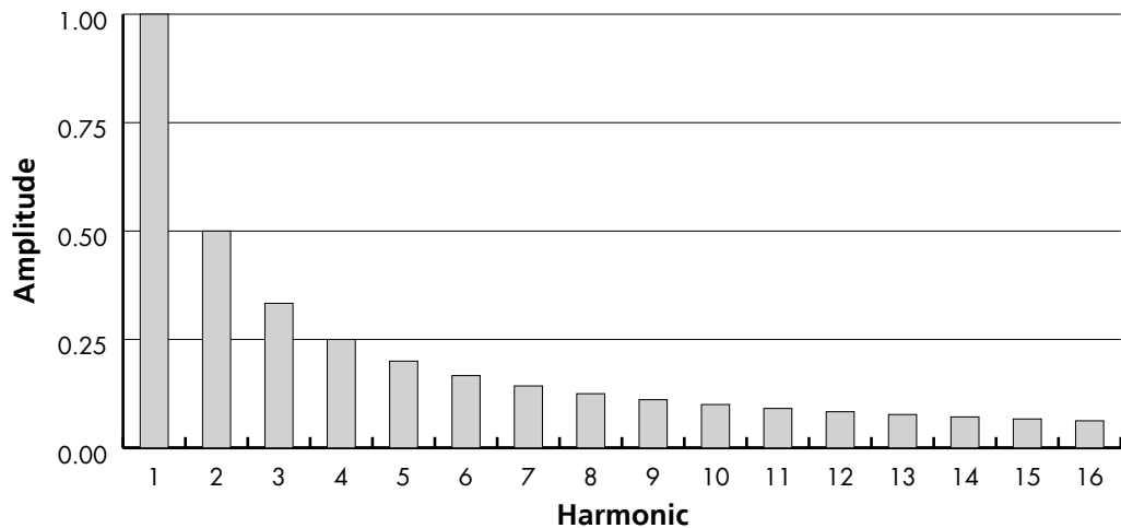
Figure 9.2 The first sixteen partials of a sawtooth wave.
