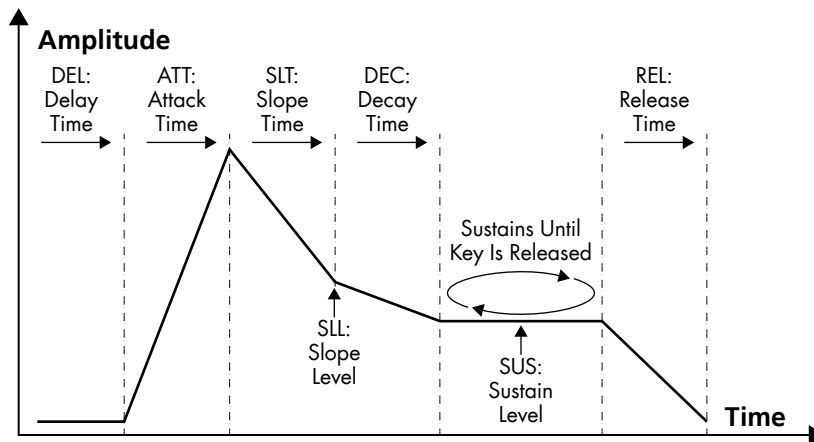
Figure 2.7 The Z3TA+ envelope offers more flexibility than the conventional ADSR envelope.
